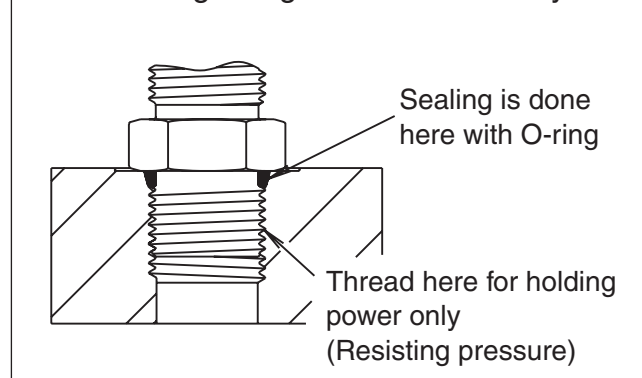
Fig. 6 – UNF port assembly
