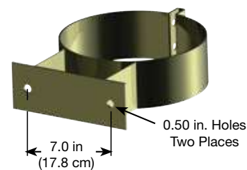
Bulkhead Mounting Bracket
